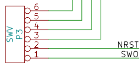
STM32 debug
