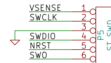
ST-style SWD
